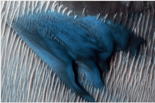
Mars 9.2.2009. Proctor Crater sand dunes. NASA|JPL-Caltech|University of Arizona
